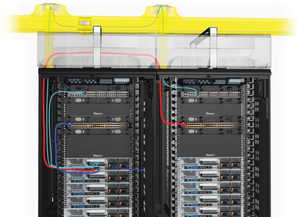
Figure 6. Single Switch – Server Cabinet Rear View
