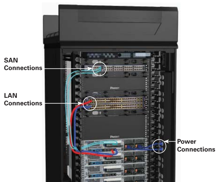
Figure 5. Dual Switch – Server Cabinet Rear View
