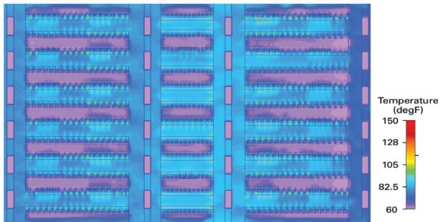
Figure 10. Data Center EoR Thermal Analysis
